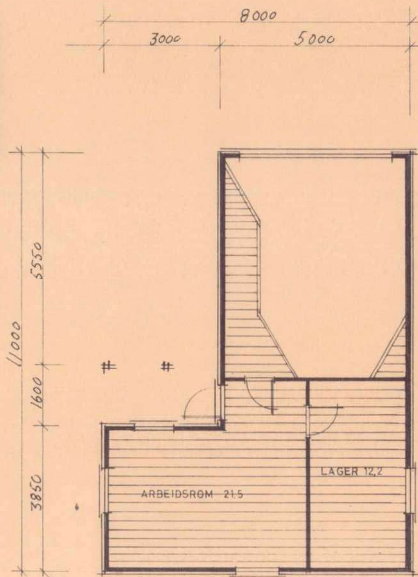
PLAN 66.5 m²
