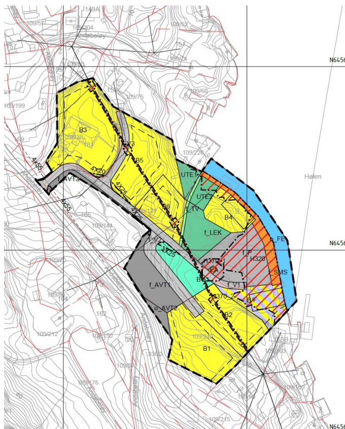
FIGUR 1: PLANKART
