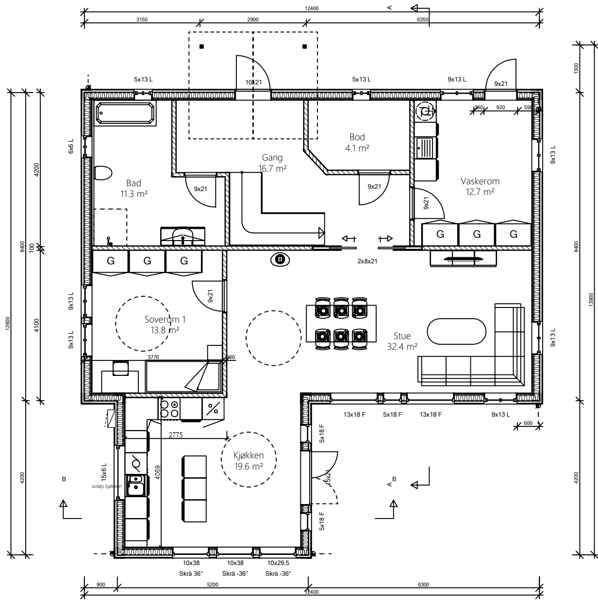
Plan 1
